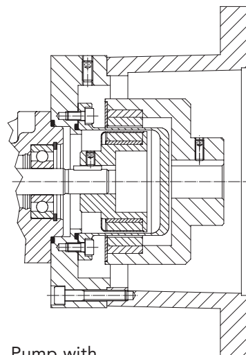
Pump with magnetic coupling
